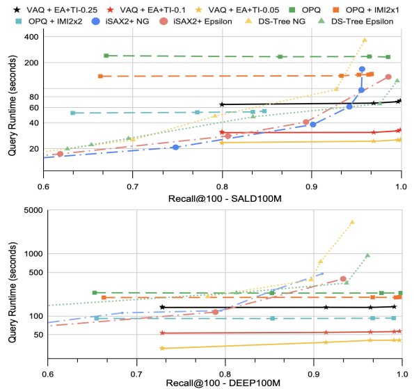
Fig. 11: Comparison of VAQ against iSAX2+, DSTree, and OPQ with indexing (OPQ+IMI variants).
