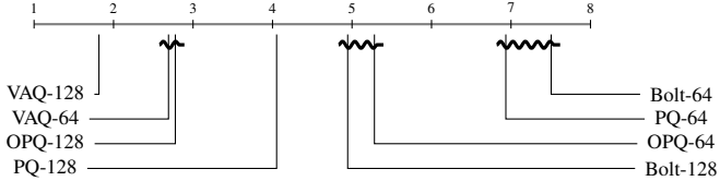
Fig. 10: Ranking of methods based on the average of their ranks across 128 datasets. The wiggly line connects all methods that do not perform statistically differently according to the Nemenyi test.
