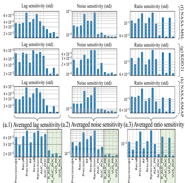
Figure 7: Robustness Analysis: over the entire benchmark, average standard deviation of the accuracy values of the measures under varying (a.1) lag, (a.2) noise, (a.3) normal/abnormal ratio. Robustness Analysis for (f) NASA-MSL, (g) KDD21 and (h) NASA-SMAP
